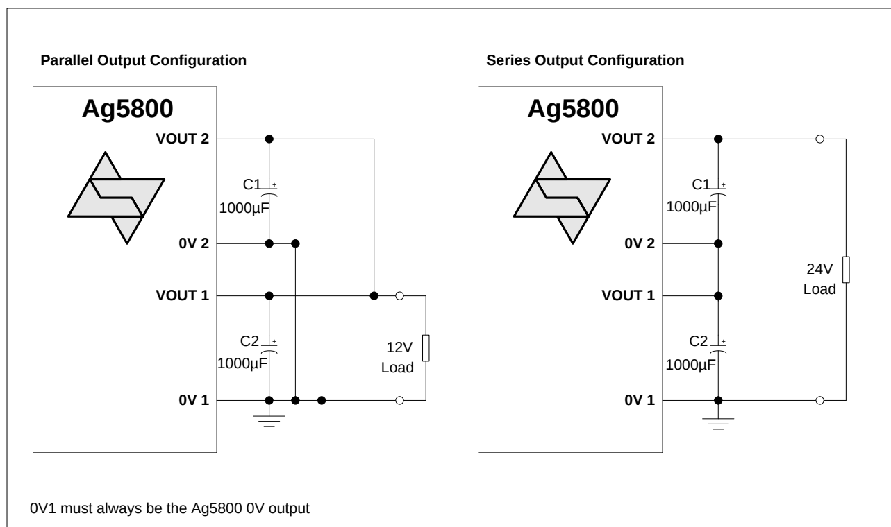
Figure 8: Output Configurations
