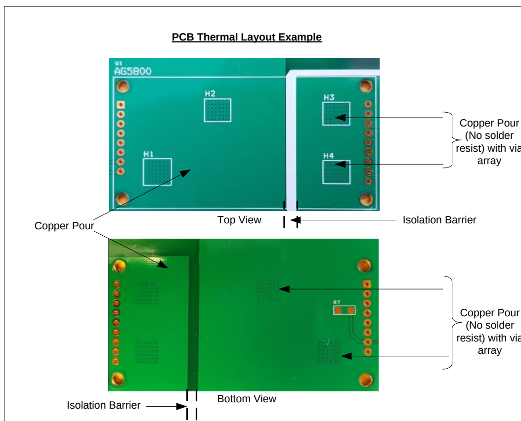
Figure 16: Suggested PCB Thermal Layout
