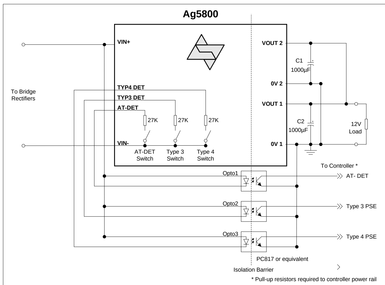
Figure 6: Physical Layer Detect Configuration
