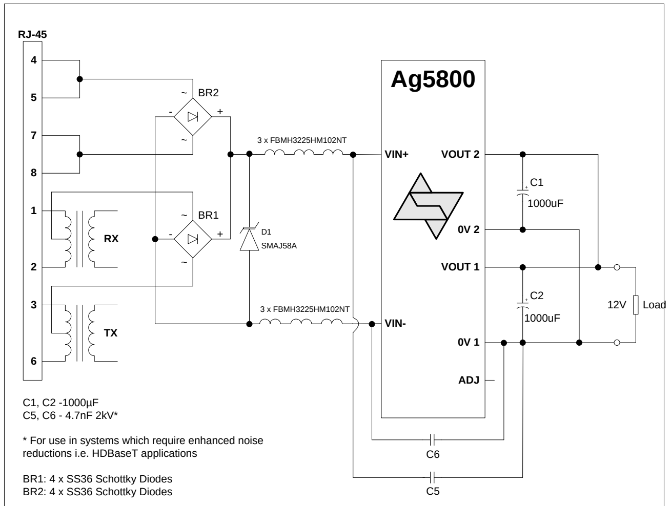
Figure 14: EMC Filtering
