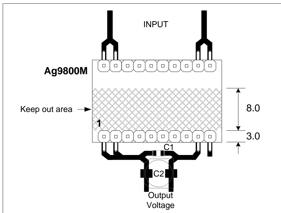
Figure 8: Layout Consideration
