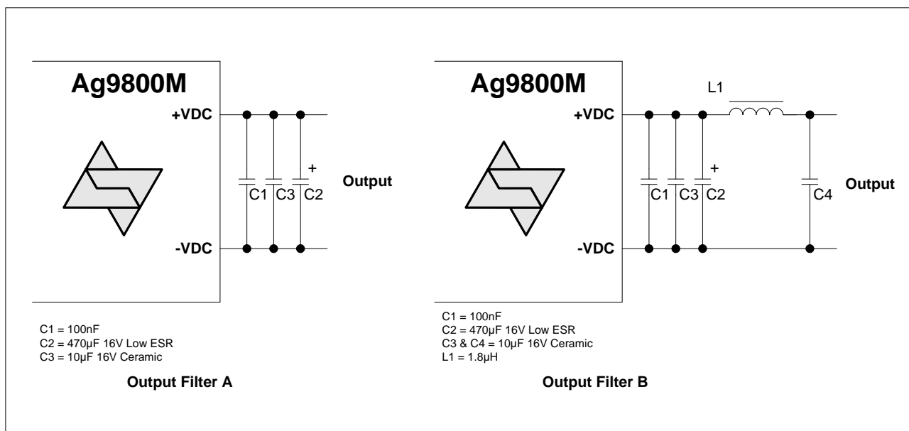
Figure 6: Output Filtering
