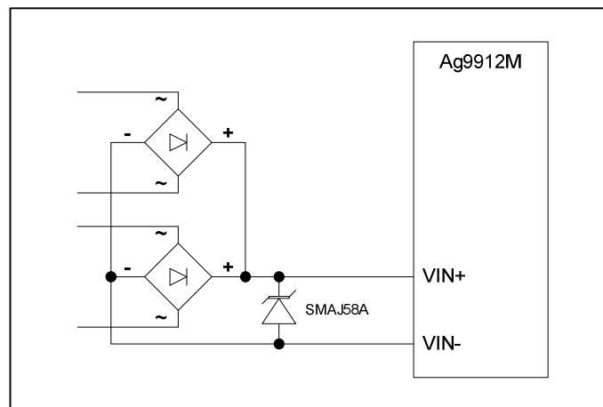
Figure 11: Ag9912M Input Protection
