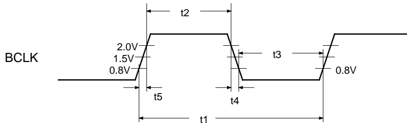
BCLK Waveform
