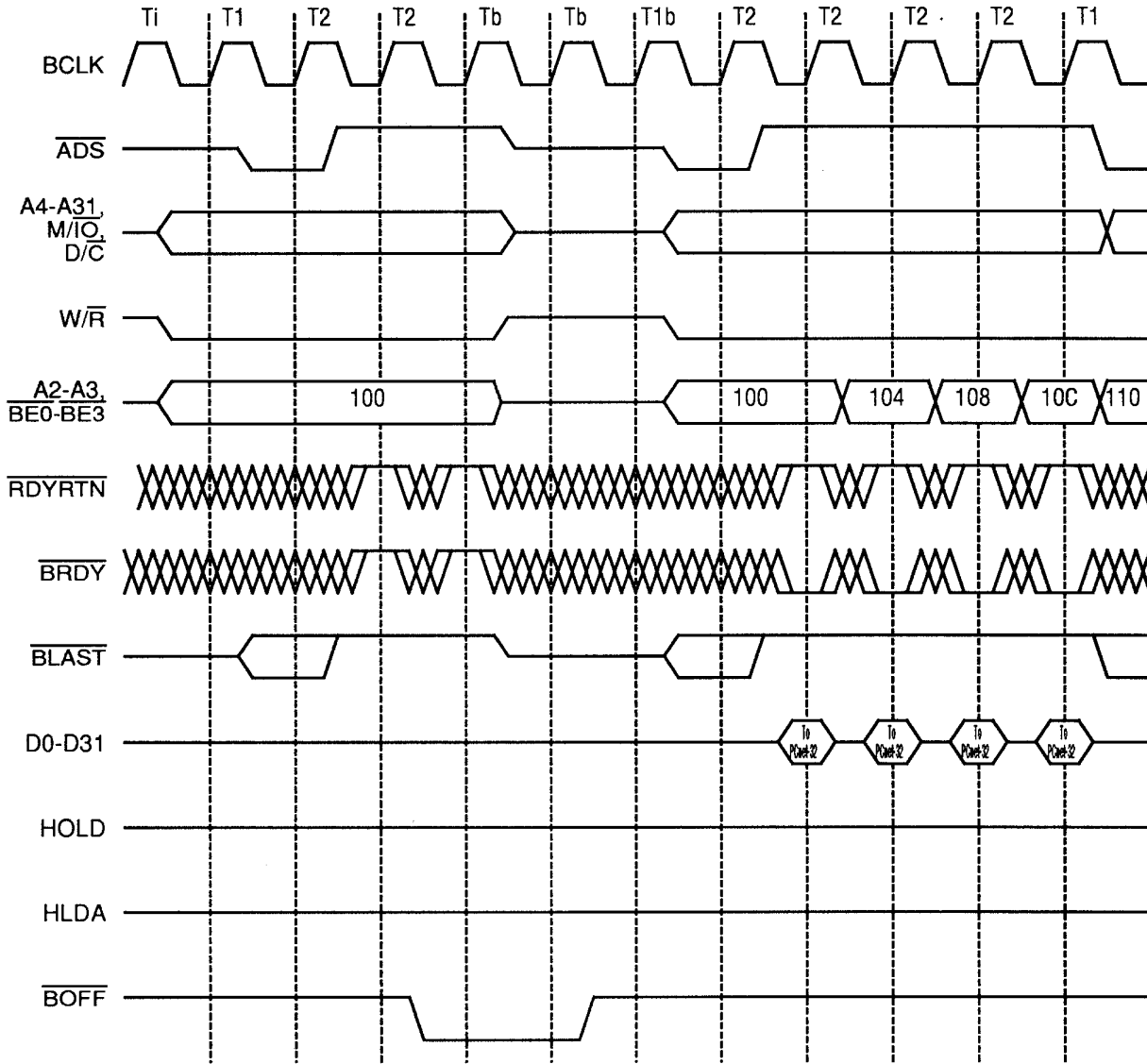
Figure 21. Restarted Linear Burst Read in which \overline{\text{BOFF}} was Asserted Before \overline{\text{BRDY}} of First Transfer in Linear Burst Sequency, Hence Linear Burst Sequence is Restarted When \overline{\text{BOFF}} is Deasserted
