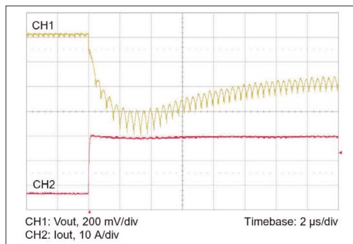
Figure 10 — 0-25 A load step with 100 \mu F input capacitor and no output capacitor.
