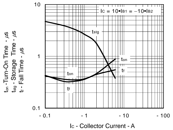
SWITCHING CHARACTERISTICS
