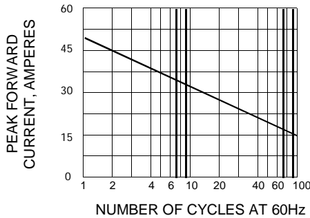
FIG.5 - MAXIMUM NON-REPETITIVE PEAK FORWARD CURRENT
