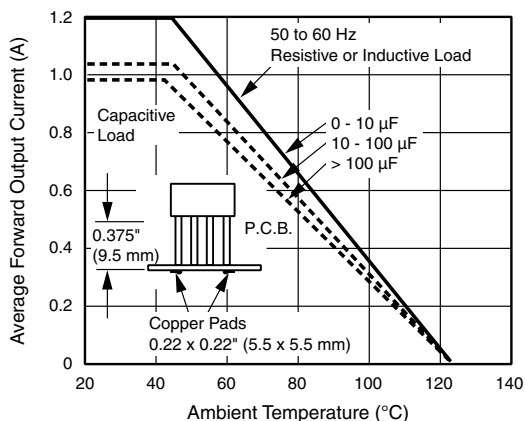
Fig. 2 - Derating Curves Output Rectified Current for B250C1000G...B380C1000G
