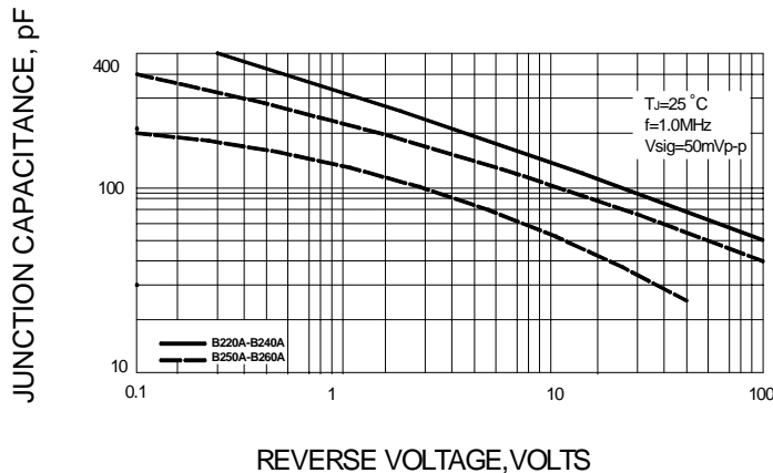
FIG.5-TYPICAL JUNCTION CAPACITANCE
