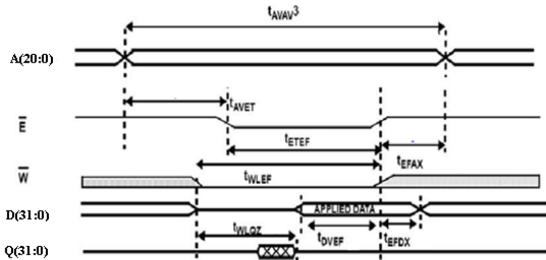
Figure 7. SRAM Write Cycle 1: \overline{W} -controlled Access
