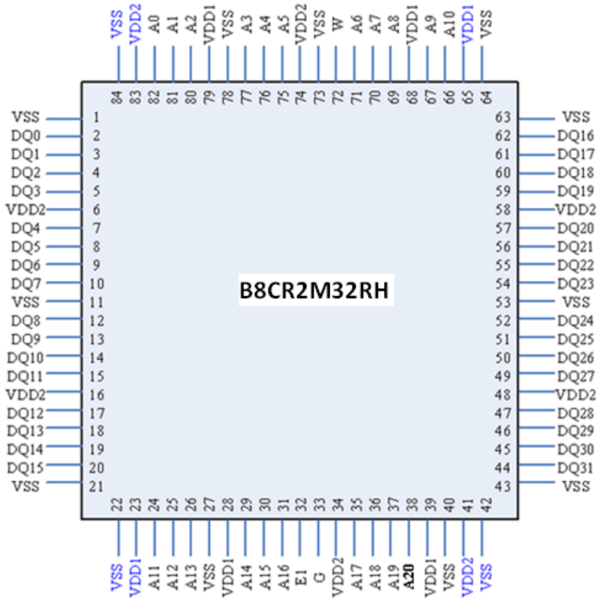
Figure 2. B8CR2M32RH SRAM Pinout
