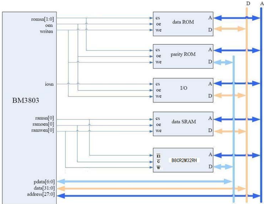
Figure 10. Typical Application
