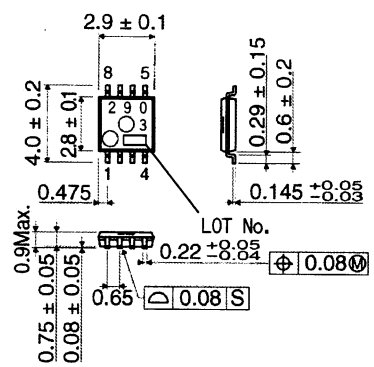
BA2903FVM(MSOP8)-(Unit:[mm])
