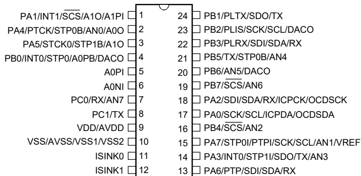
BA45F5250/BA45V5250 24 SSOP-A
