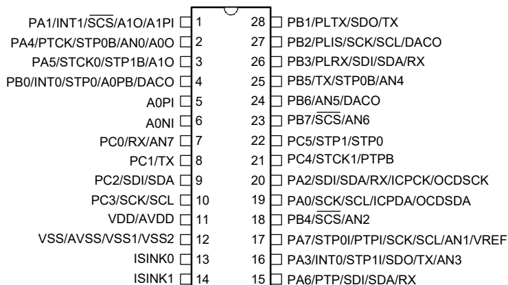
BA45F5250/BA45V5250 28 SSOP-A
