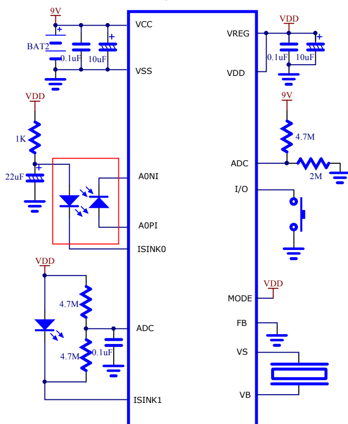
External-Driving Buzzer Application Circuit
