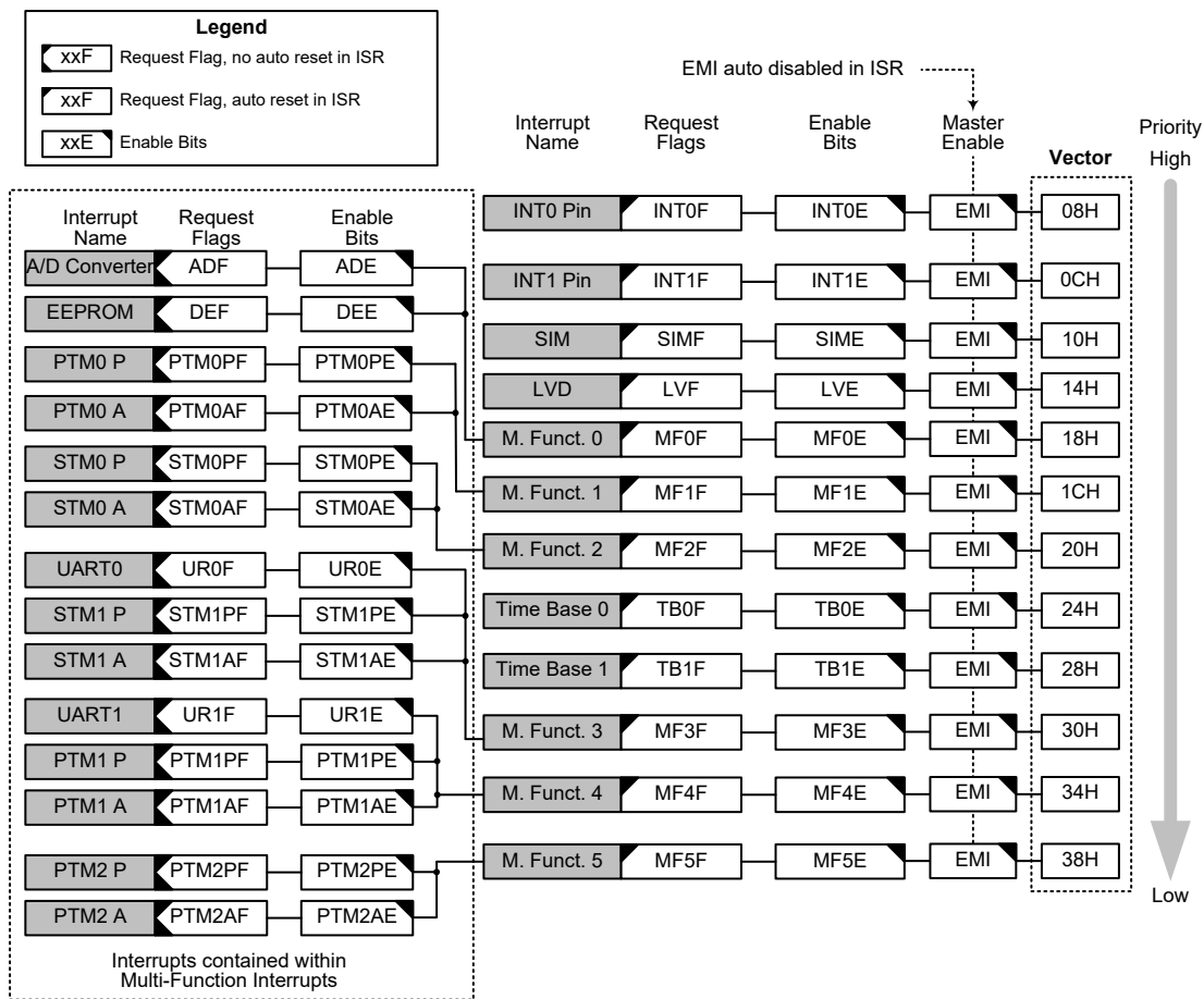
Interrupt Structure
