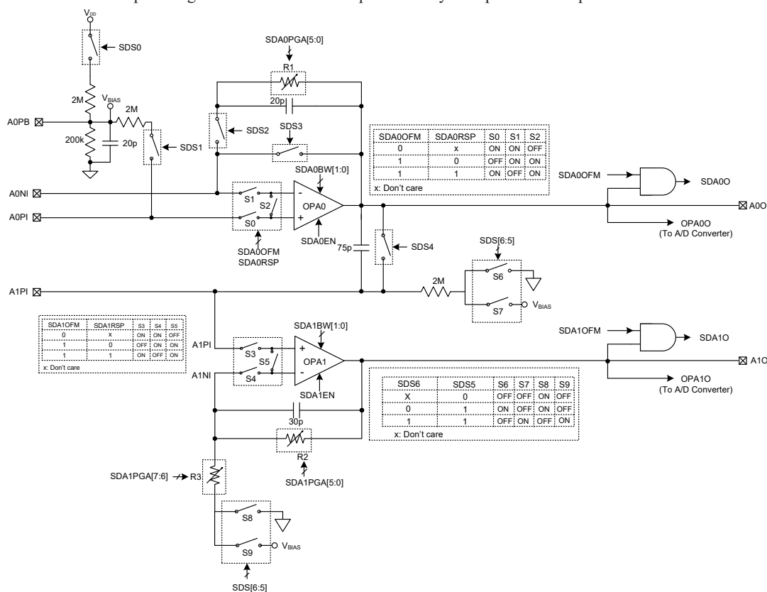
Smoke Detector AFE Block Diagram
