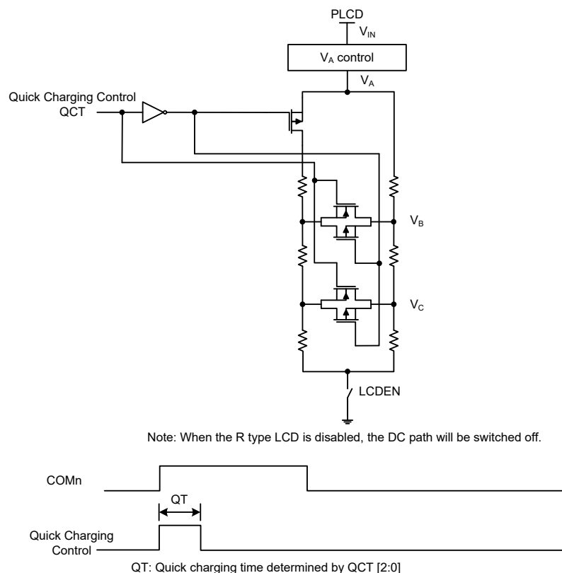
R Type Bias Configuration – 1/3 Bias
