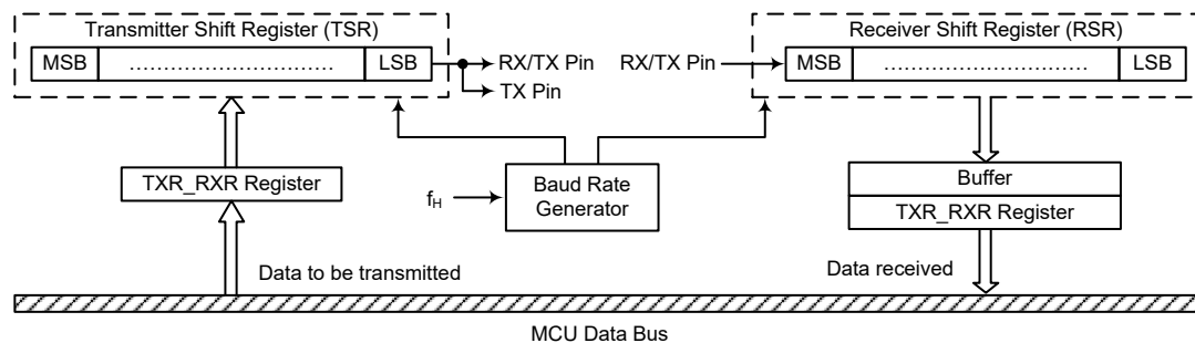
UART Data Transfer Block Diagram – SWM=1
