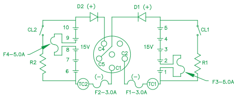
ELECTRICAL SCHEMATIC
