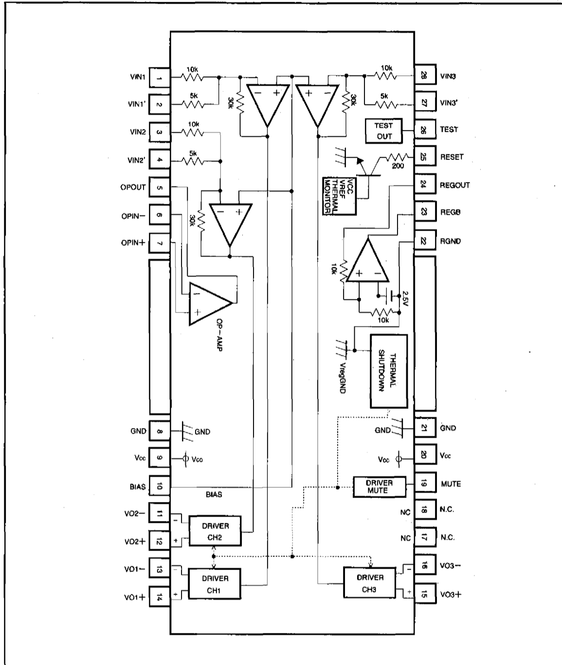
●Block diagram
