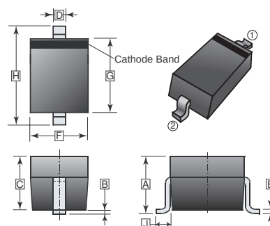
SOD-323
