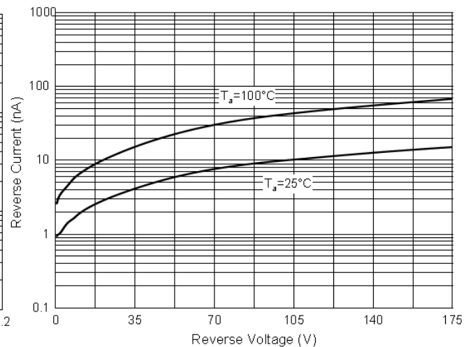
Fig. 2 - Reverse Characteristics
