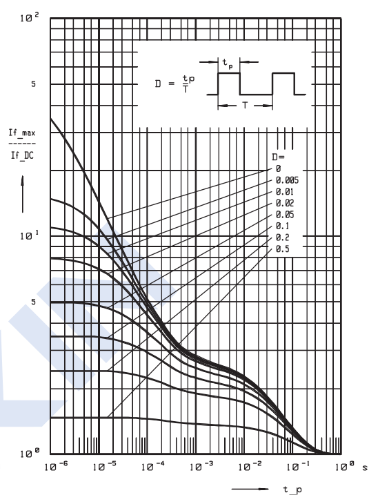
Permissible pulse load I_{fmax}/I_{fDC} = f(t_p) BAR64W
