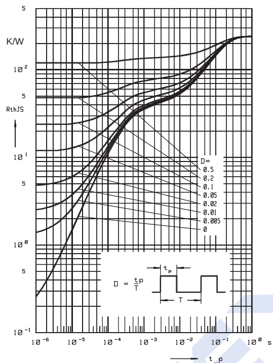
Permissible pulse load R_{thJS} = f(t_p) BAR64W
