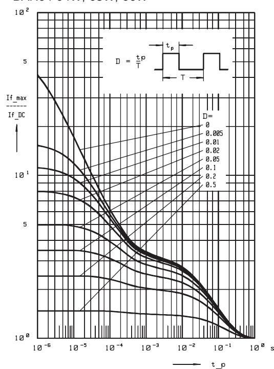
Permissible pulse load I_{fmax}/I_{fDC} = f(t_p) BAR64-04W, -05W, -06W
