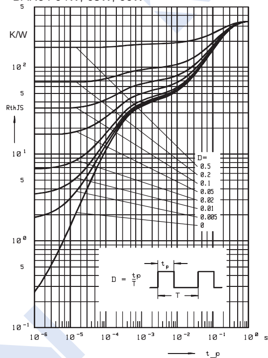
Permissible pulse load R_{thJS} = f(t_p) BAR64-04W, -05W, -06W
