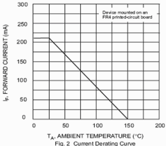
Fig. 2 Current Derating Curve
