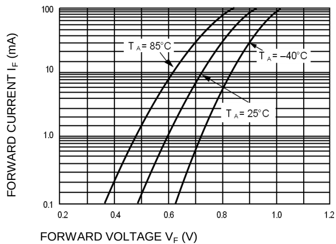
Fig 1 Forward Voltage
