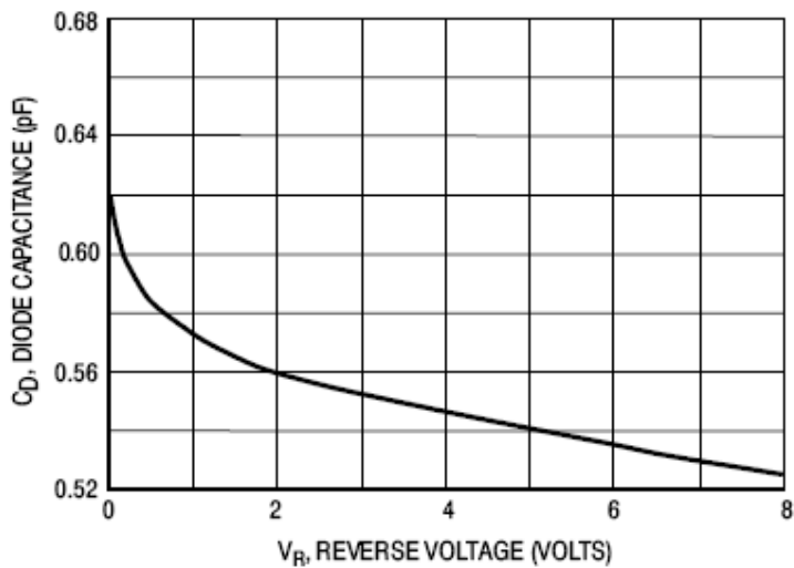
Figure 4. Capacitance
