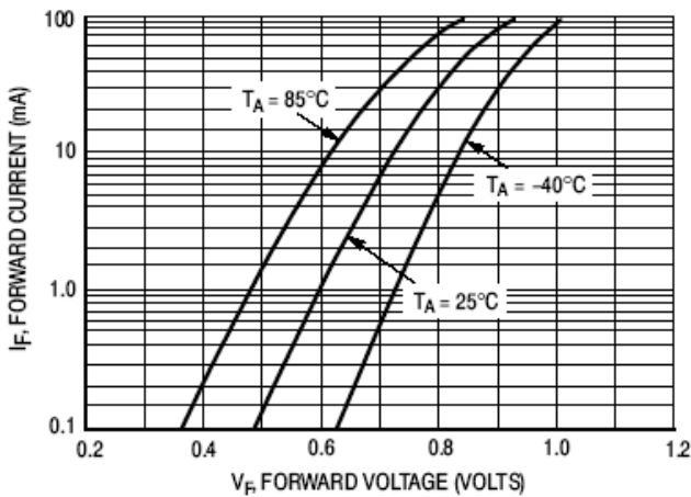
Figure 2. Forward Voltage
