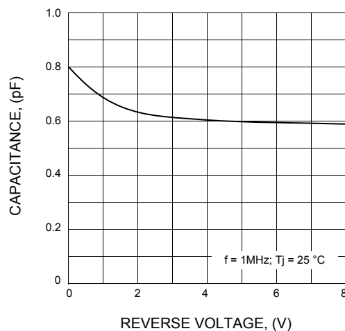
FIG.2 - DIODE CAPACITANCE VS. REVERSE VOLTAGE; TYPICAL VALUES
