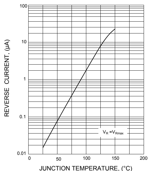
FIG.4 - REVERSE CURRENT VS. JUNCTION TEMPERATURE; TYPICAL VALUES
