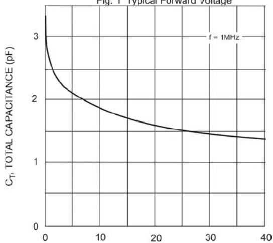
Fig. 3 Typical Capacitance
