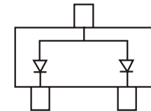
BAS40W-06 Marking: K46
