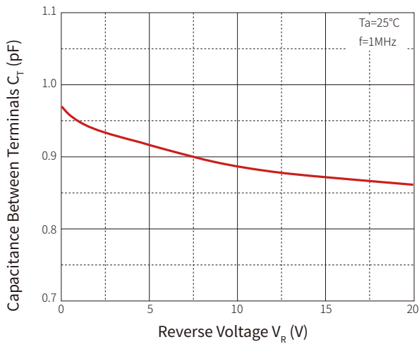
Fig.3 Capacitance Characteristics
