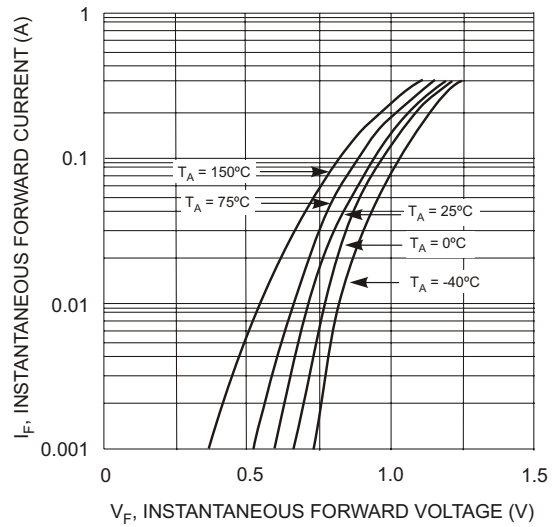
Fig. 2 Forward Characteristics
