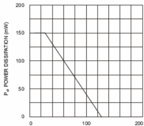
Fig. 4 Power Derating Curve, Total Package
