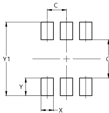
SOT363 (Standard)
