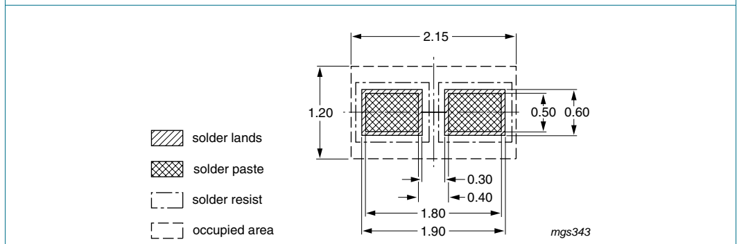
Fig 15. Wave soldering footprint SOD323 (SC-76)
