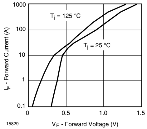
15829 Figure 3. Forward Current vs. Forward Voltage
