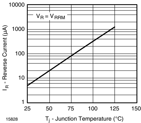
15828 Figure 2. Reverse Current vs. Junction Temperature
