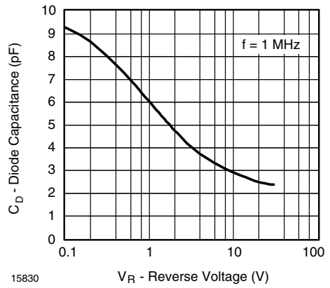
15830 Figure 4. Diode Capacitance vs. Reverse Voltage
