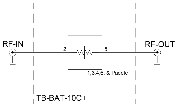
Figure 2. BAT-10+ Characterization and Application Circuit.
