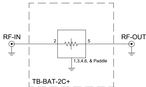
Figure 2. BAT-2+ Characterization and Application Circuit.
