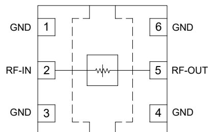
Figure 1. BAT-30+ Functional Diagram
