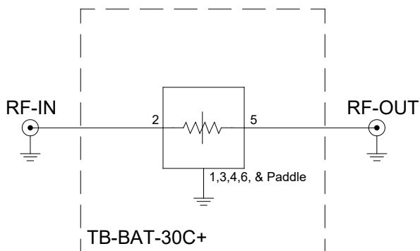
Figure 2. BAT-30+ Characterization and Application Circuit.
