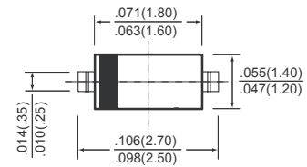
SOD-323
