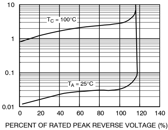
Figure 3. Reverse Characteristics
