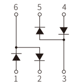
Schematic Symbol
