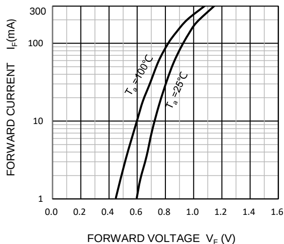
Forward Characteristics
