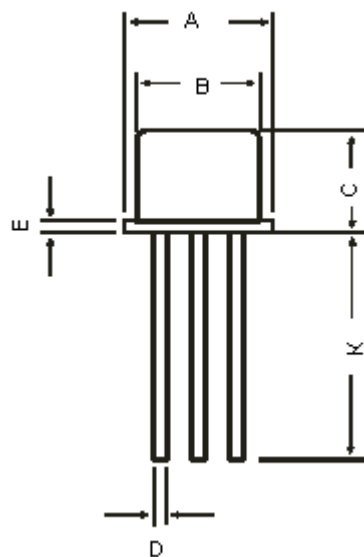
TO-18 Metal Can Package
