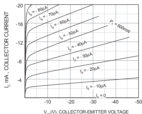
Fig.2 Static Characteristic
