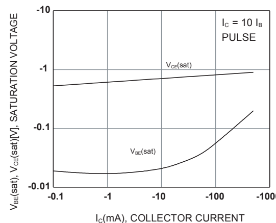
Fig.4 Base-Emitter Saturation Voltage Collector-Emitter Saturation Voltage
