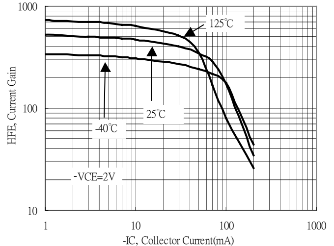
Current gain vs Collector Current
