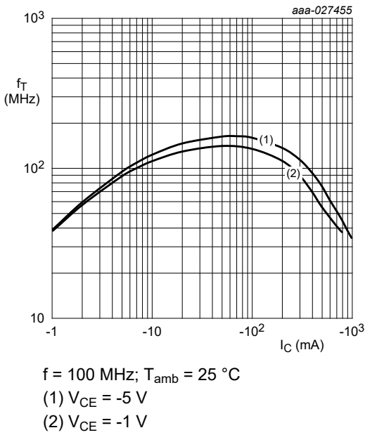
Fig. 30. BC807K-25-Q: Transition frequency as a function of collector current; typical values
