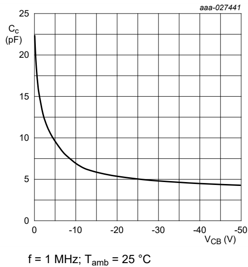
Fig. 16. BC807K-16-Q: Collector capacitance as a function of collector-base voltage; typical values
