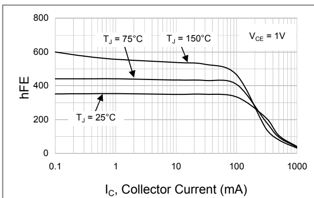
Fig.5 BC817-40W-AU : DC Current Gain
