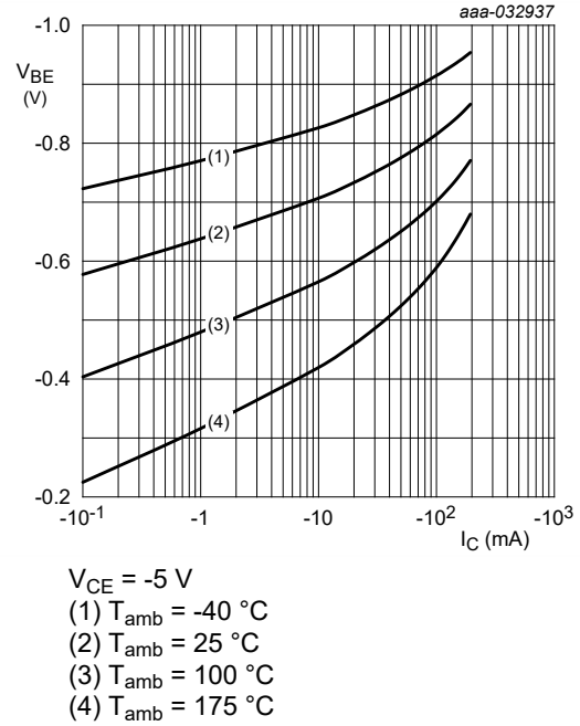
Fig. 12. TR2 (PNP): Base-emitter voltage as a function of collector current; typical value
