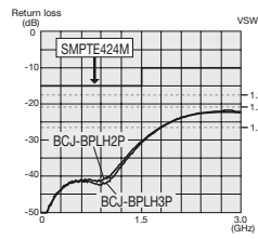
Return loss for BCJ-BPLH2P, BCJ-BPLH3P
