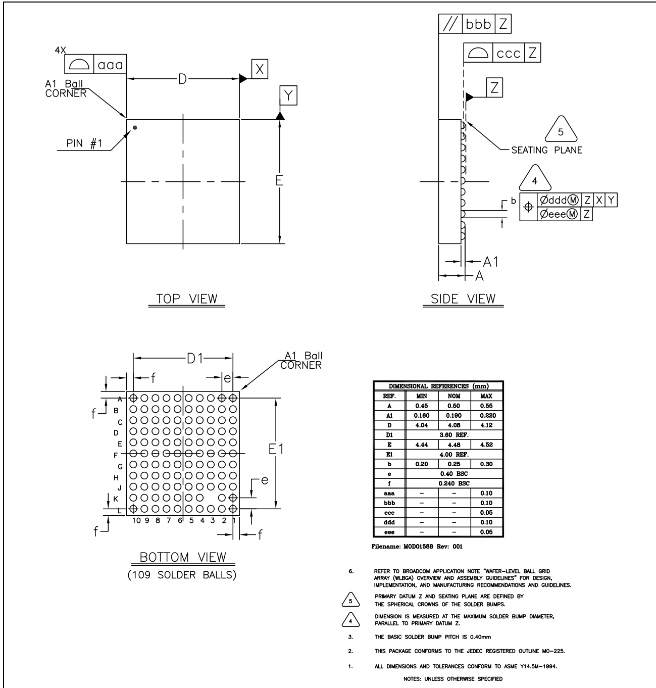
Figure 49: 109-Ball WLBGA Package Mechanical Information
