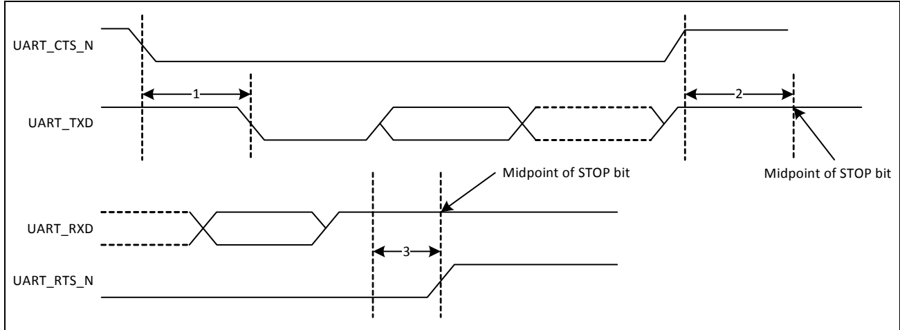
Figure 17: UART Timing
