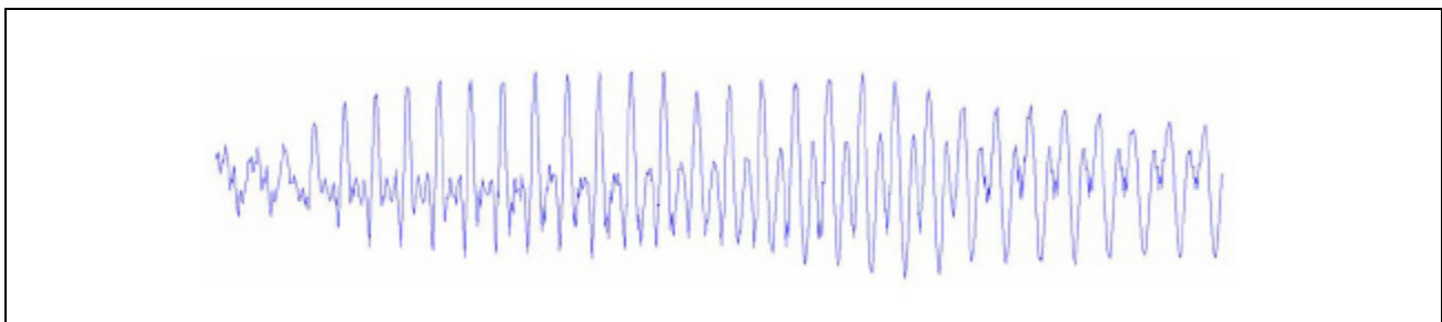
Figure 10: CVSD Decoder Output Waveform After Applying PLC
