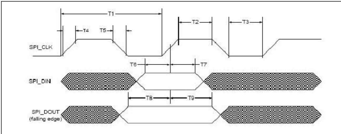
Figure 44: gSPI Timing
