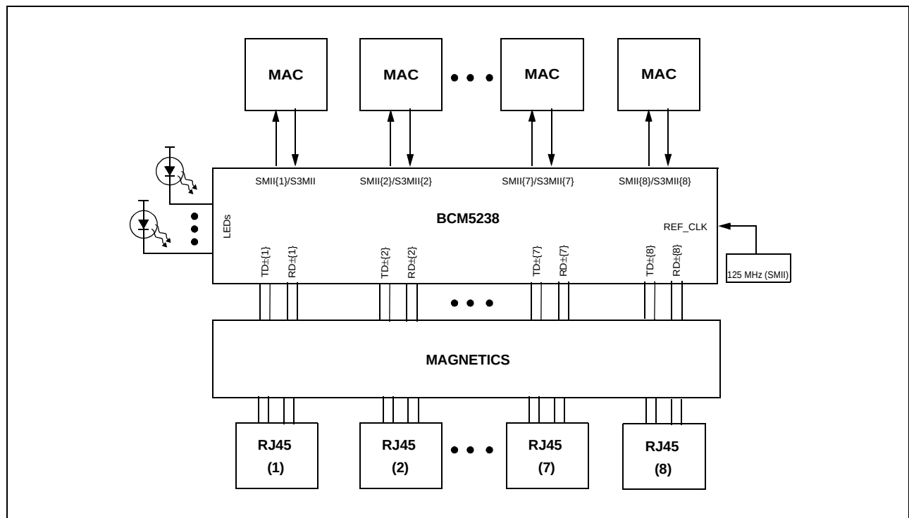
Figure 12: Switch Application
