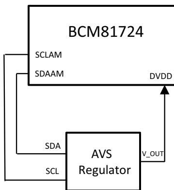
Figure 4: AVS Configuration (One Regulator for One Package)
