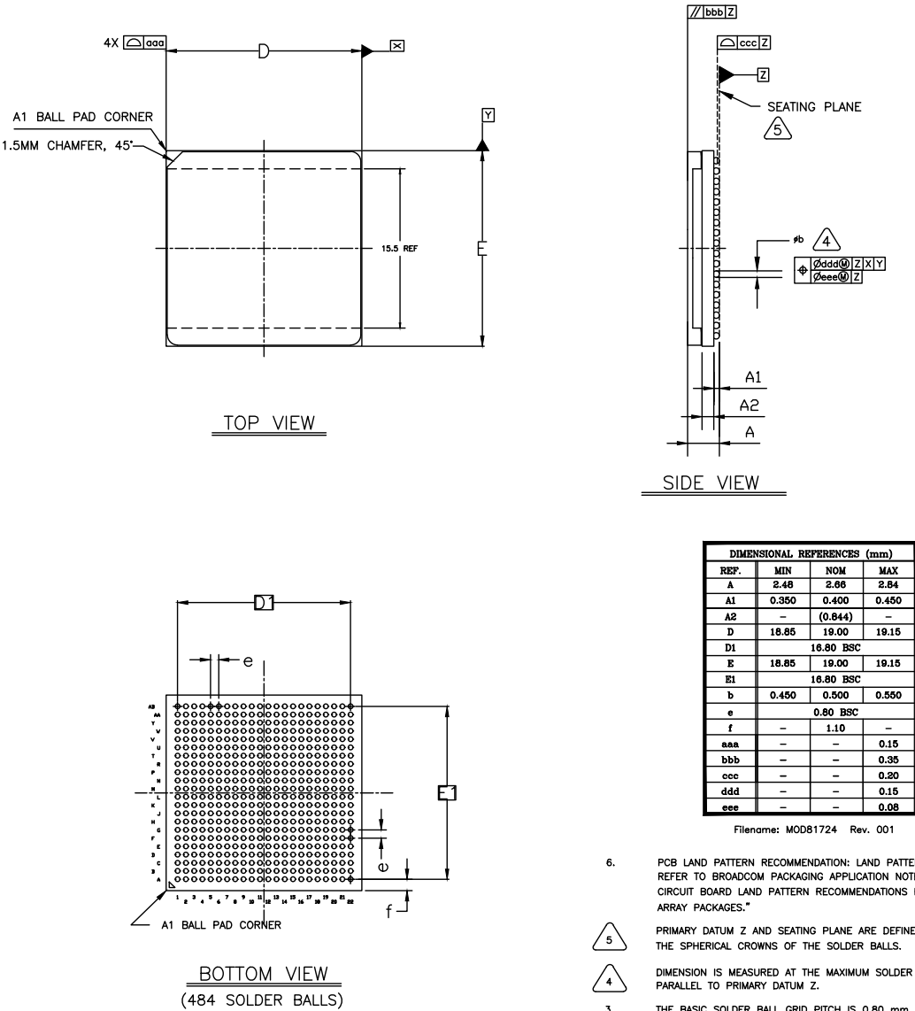
Figure 15: 19 mm × 19 mm, 484-Ball BGA, RoHS-Compliant Package
